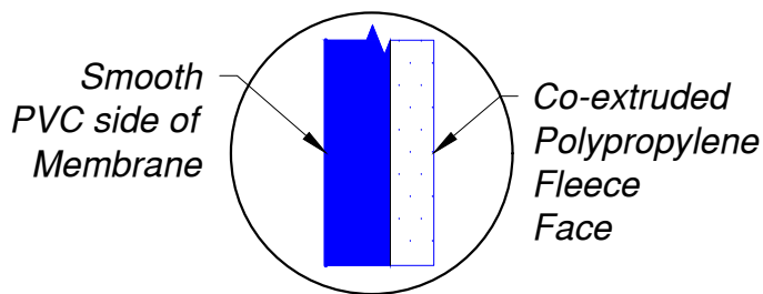
DualProof C Membrane Cross-section
